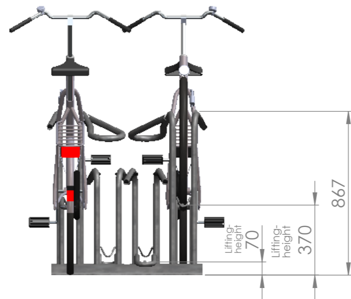
K1252, Mamba 4D double-sided - h.2.h. 400 mm
